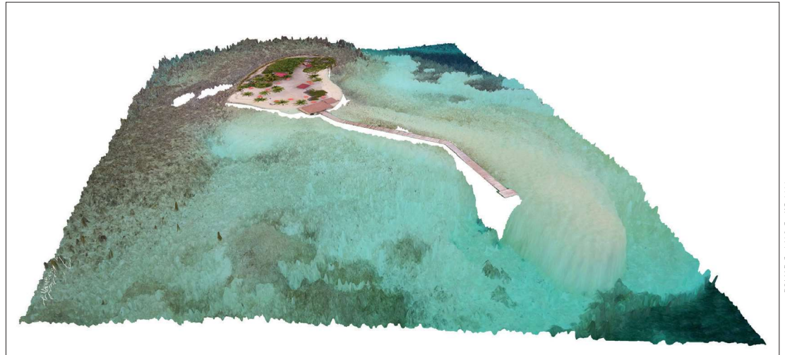
Fig. 3: Combining drone- and satellite-analysis for mapping shallow water environments. The example shows an area of approximately 250 × 250 m in Belize and represents depth at 9 cm spatial resolution overlaid with a real-colour image which shows the different seafloor types from bright sand to coral and hardbottom areas (top left) to sparse to dense seagrass areas (lower right and centre)
